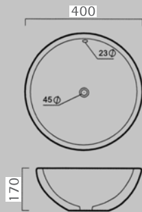
2 E-7004 400x400x170 mm Tezgah üstü lavabo Over-the-counter basin
