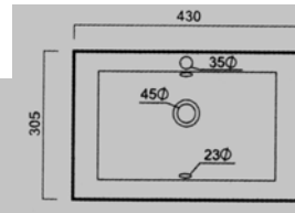
3 E-4128 430x305x135 mm Tezgah üstü lavabo Over-the-counter basin
