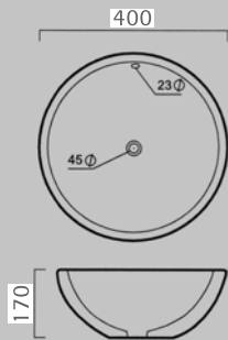
1 E-7003 400x400x170 mm Tezgah üstü lavabo Over-the-counter basin
