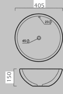
4 E-7006 405x405x150 mm Tezgah üstü lavabo Over-the-counter basin
