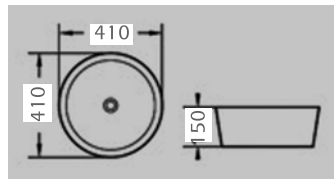
1 E-8202 410x410x150 mm Tezgah üstü lavabo Over-the-counter basin
