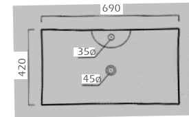
4 E-4145 690x420x130 mm Tezgah üstü lavabo Over-the-counter basin
